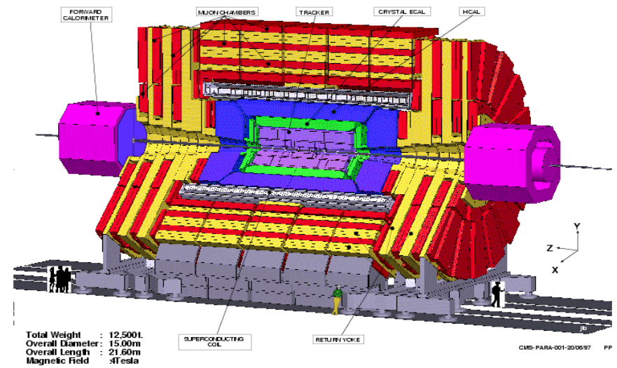
CMS
