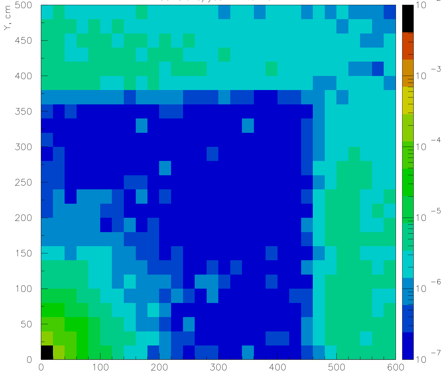
MUON St.2 charged hadrons, particle/collision/cm 2
