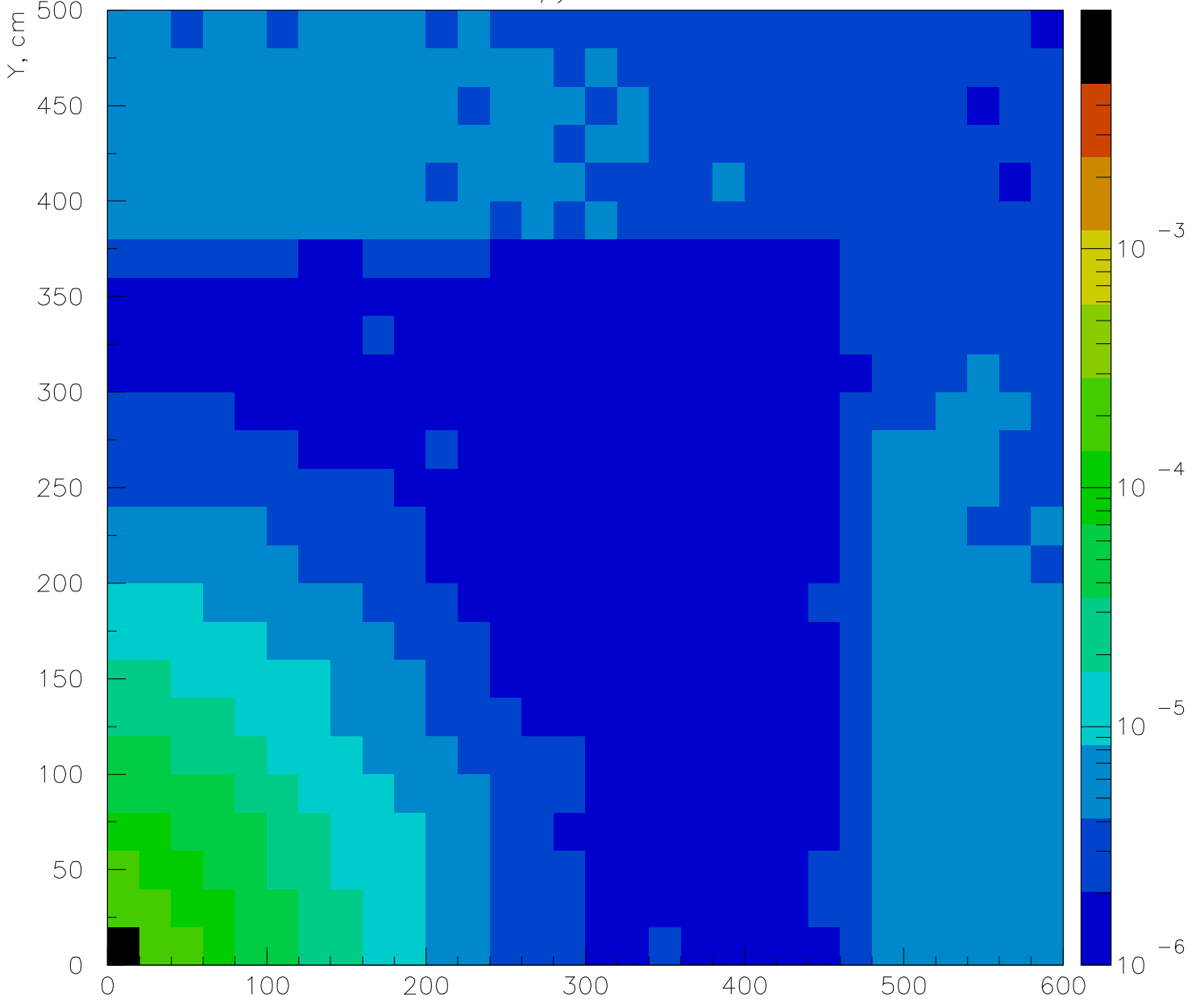
MUON St.2 hadrons ( E \geq 20 MeV), particle/collision/ \text{cm}^2
