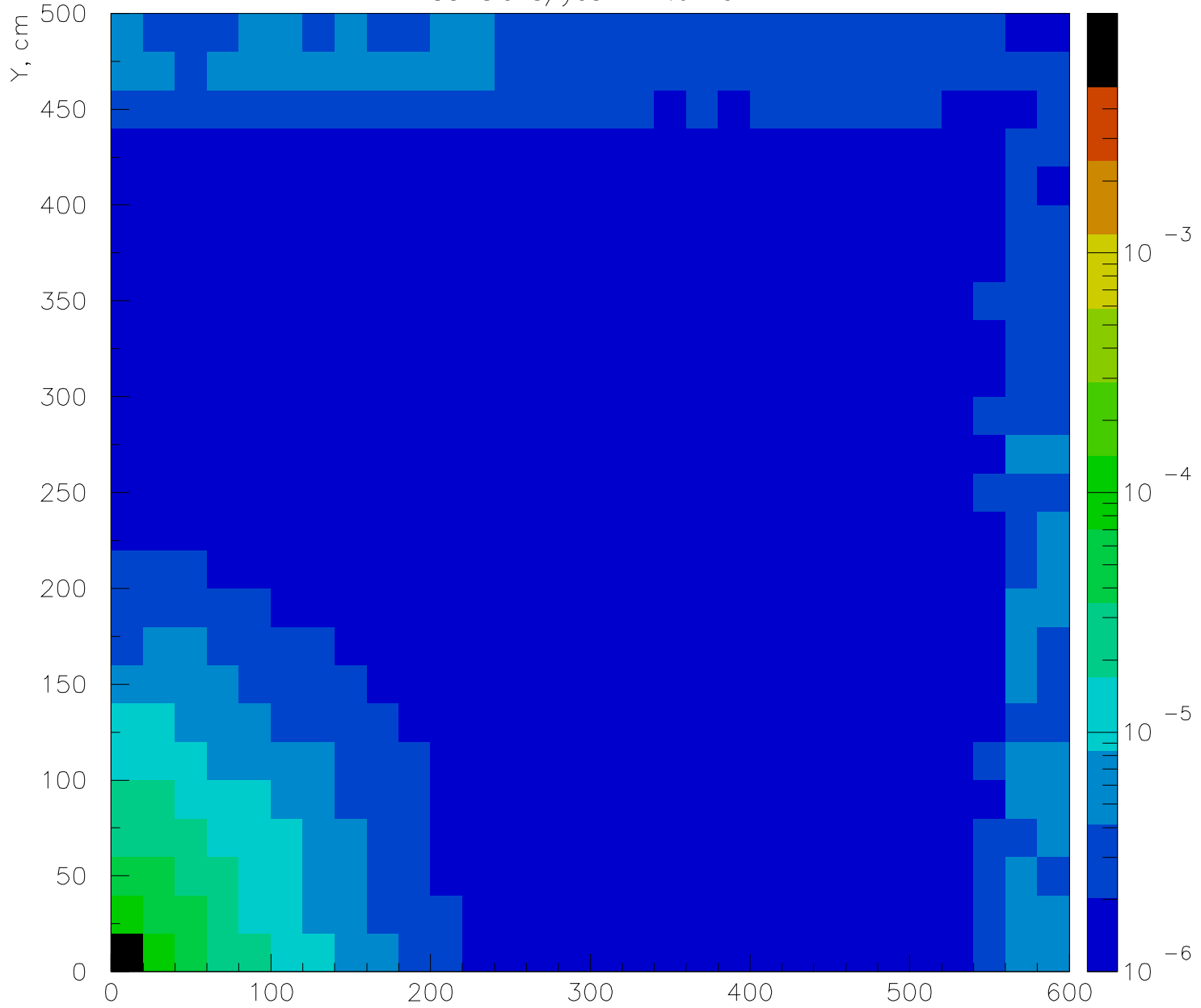
MUON St.3 hadrons (E ge 20MeV), particle/collision/cm 2
