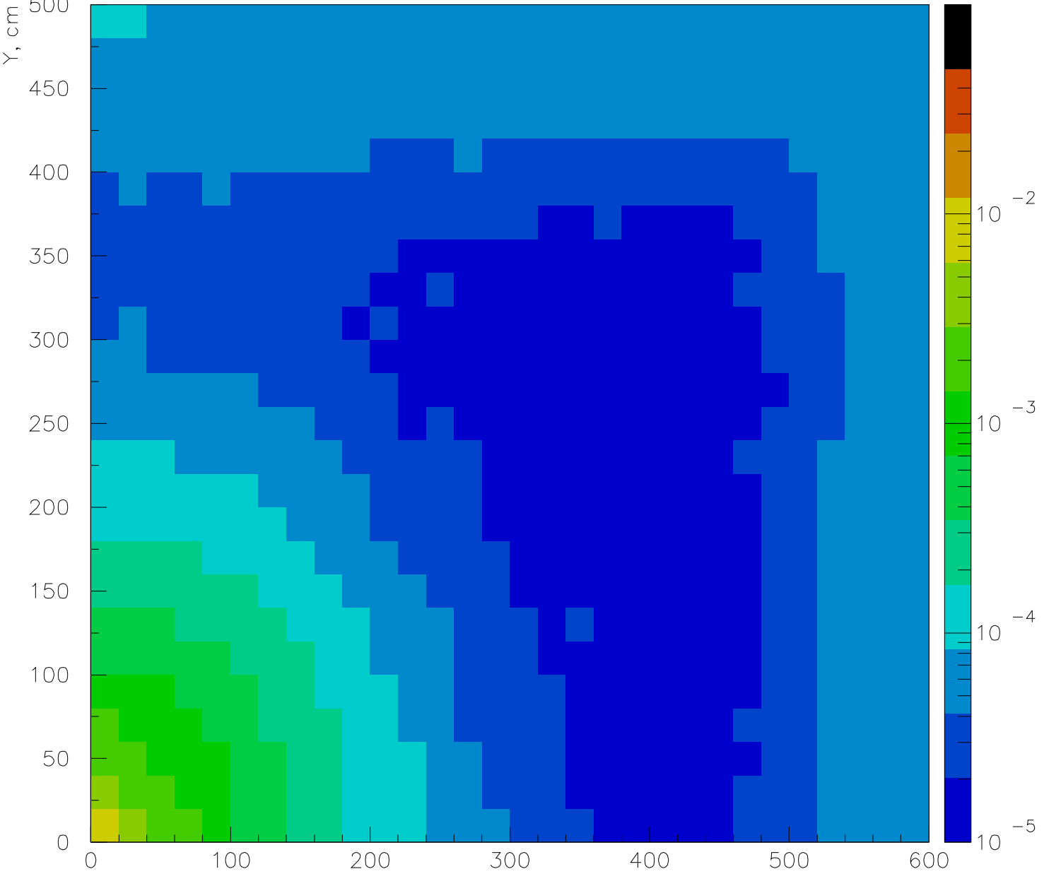
MUON St.3 1MeV neutrons eqv. fluence, particle/collision/cm 2
