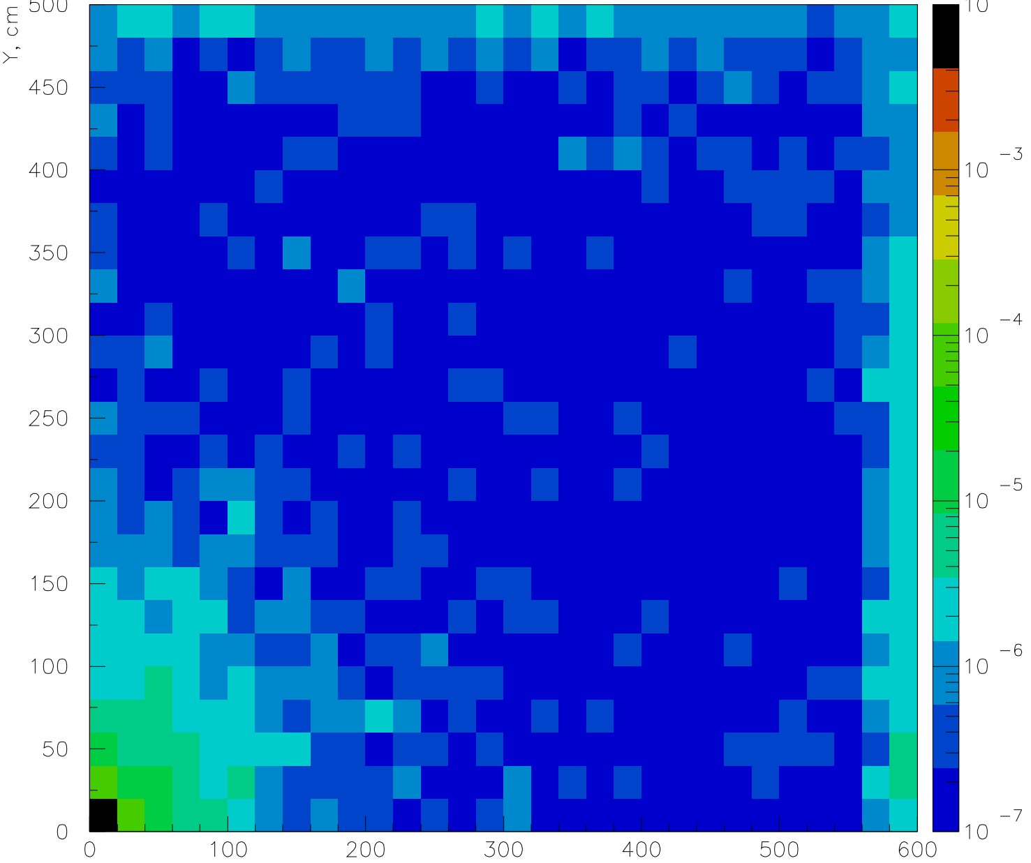
MUON St.4 electrons-positrons, particle/collision/cm 2
