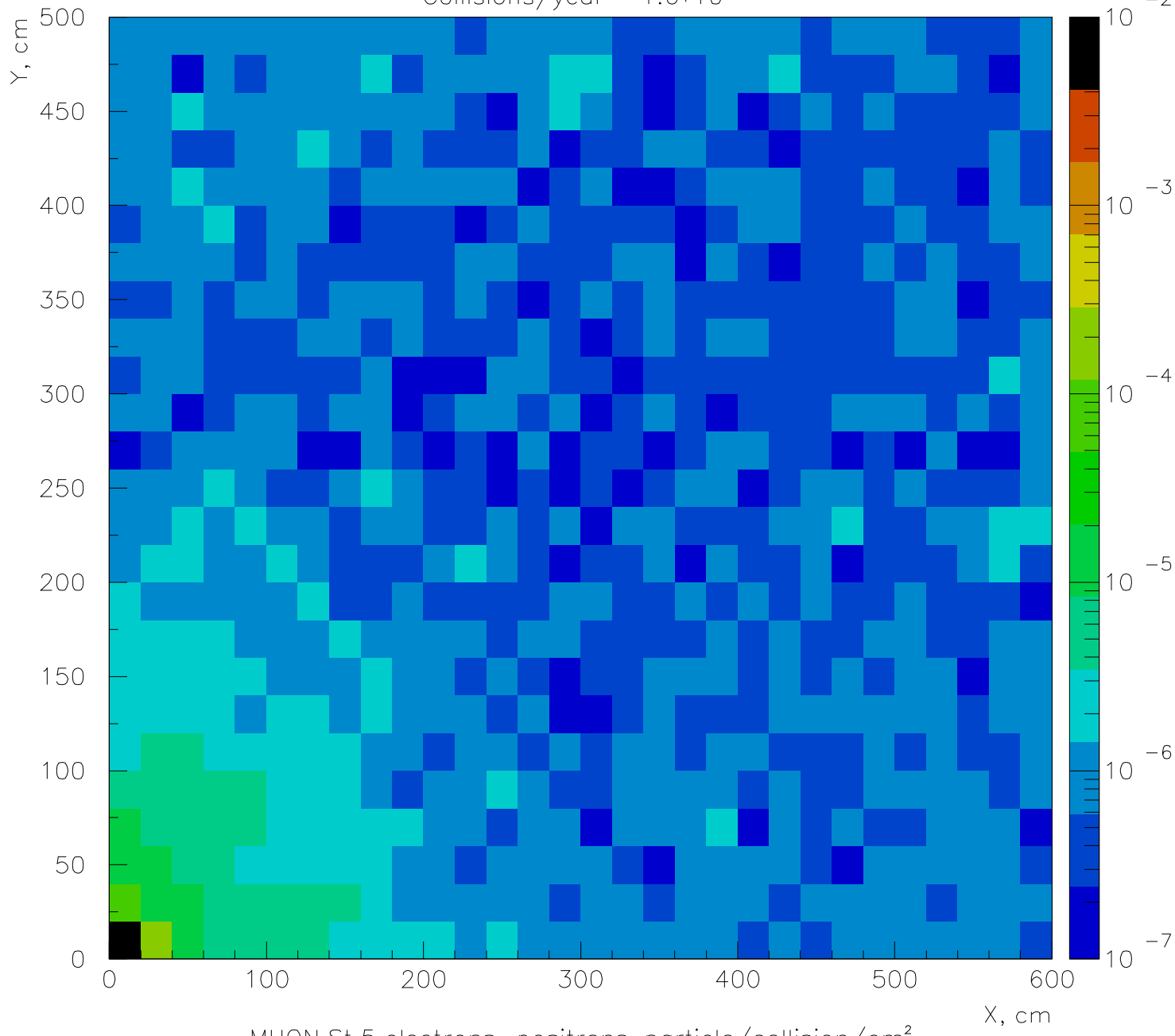
MUON St.5 electrons-positrons, particle/collision/cm 2
