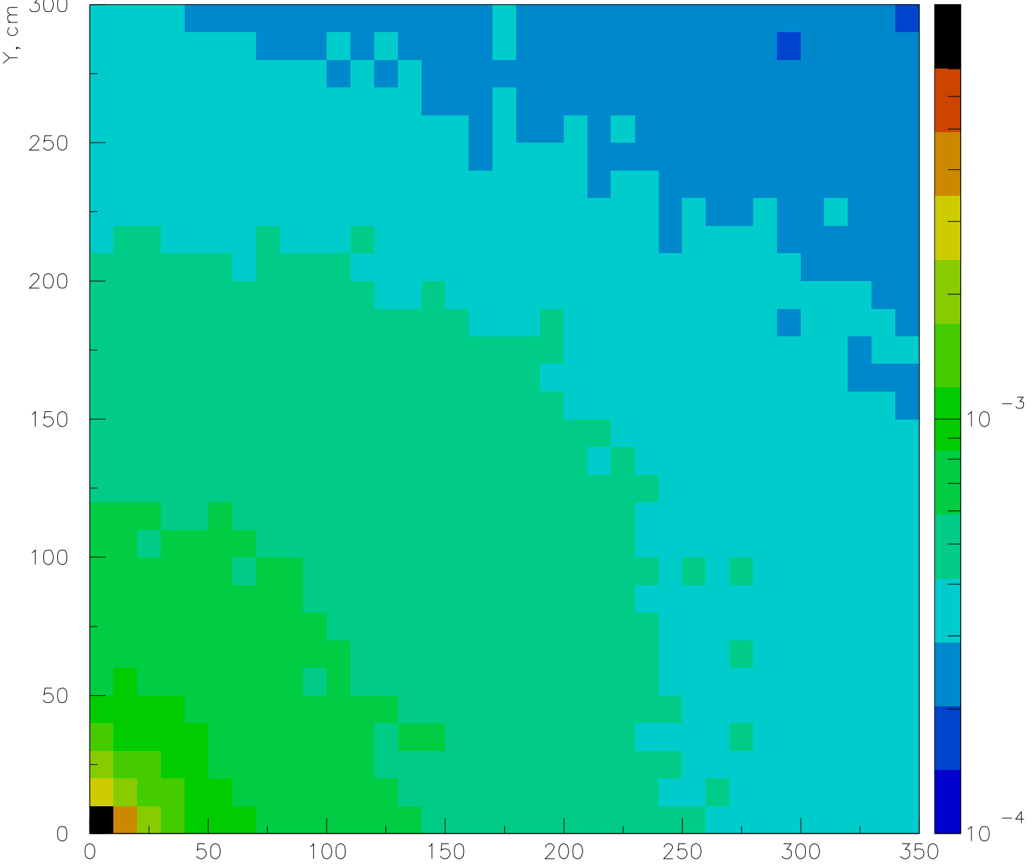
OT St.T1 1MeV neutrons eqv. fluence, particle/collision/cm 2
