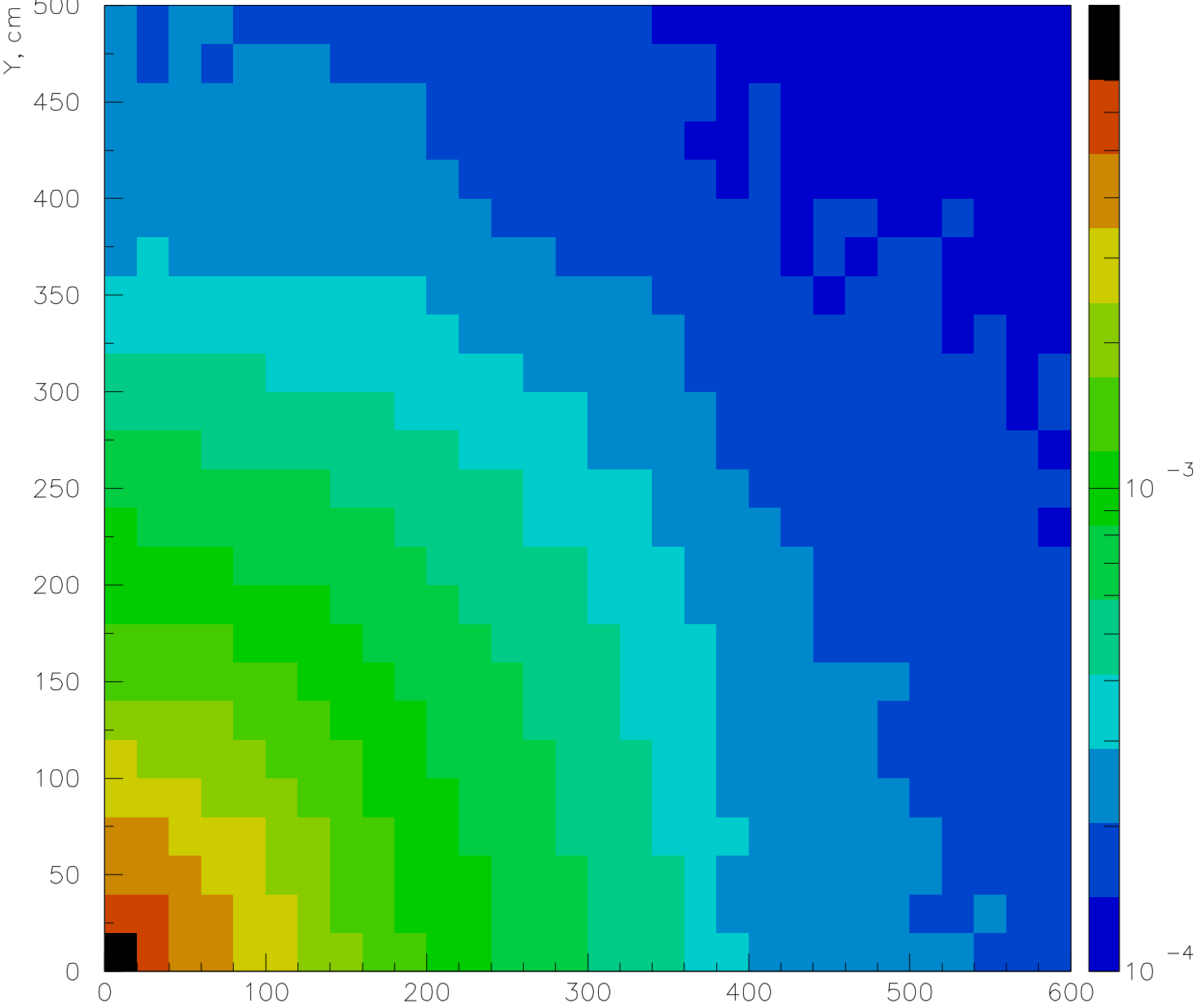
RICH 2 1MeV neutrons eqv. fluence, particle/collision/cm 2
