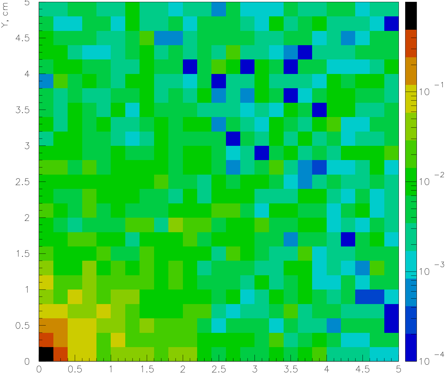
sensor Z=0cm neutrons, particle/collision/cm 2
