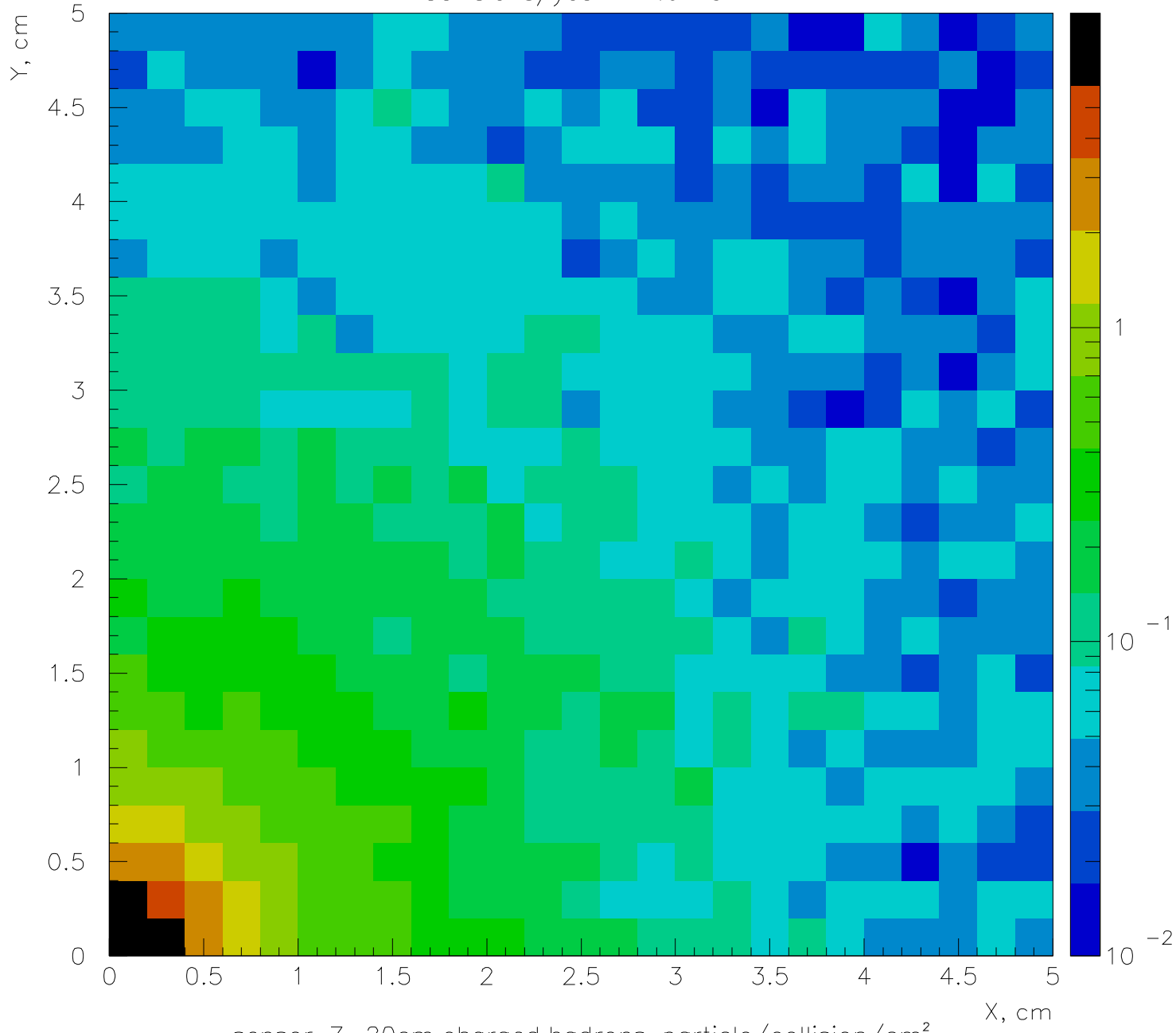
sensor Z=20cm charged hadrons, particle/collision/cm 2
