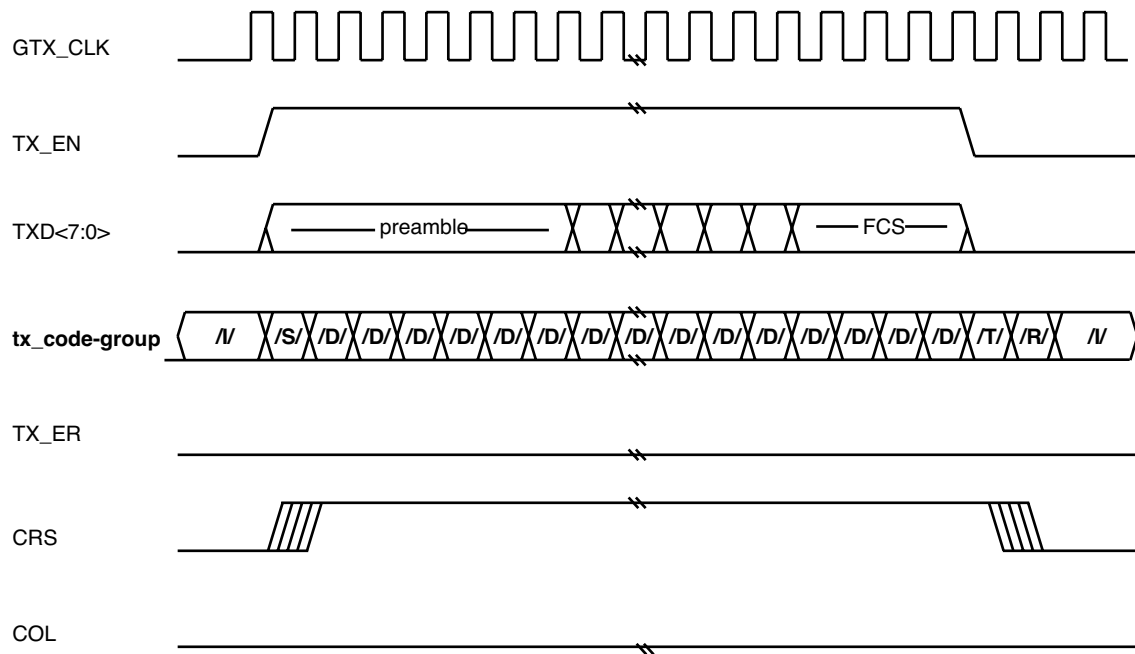
Figure 36-4—PCS encapsulation
