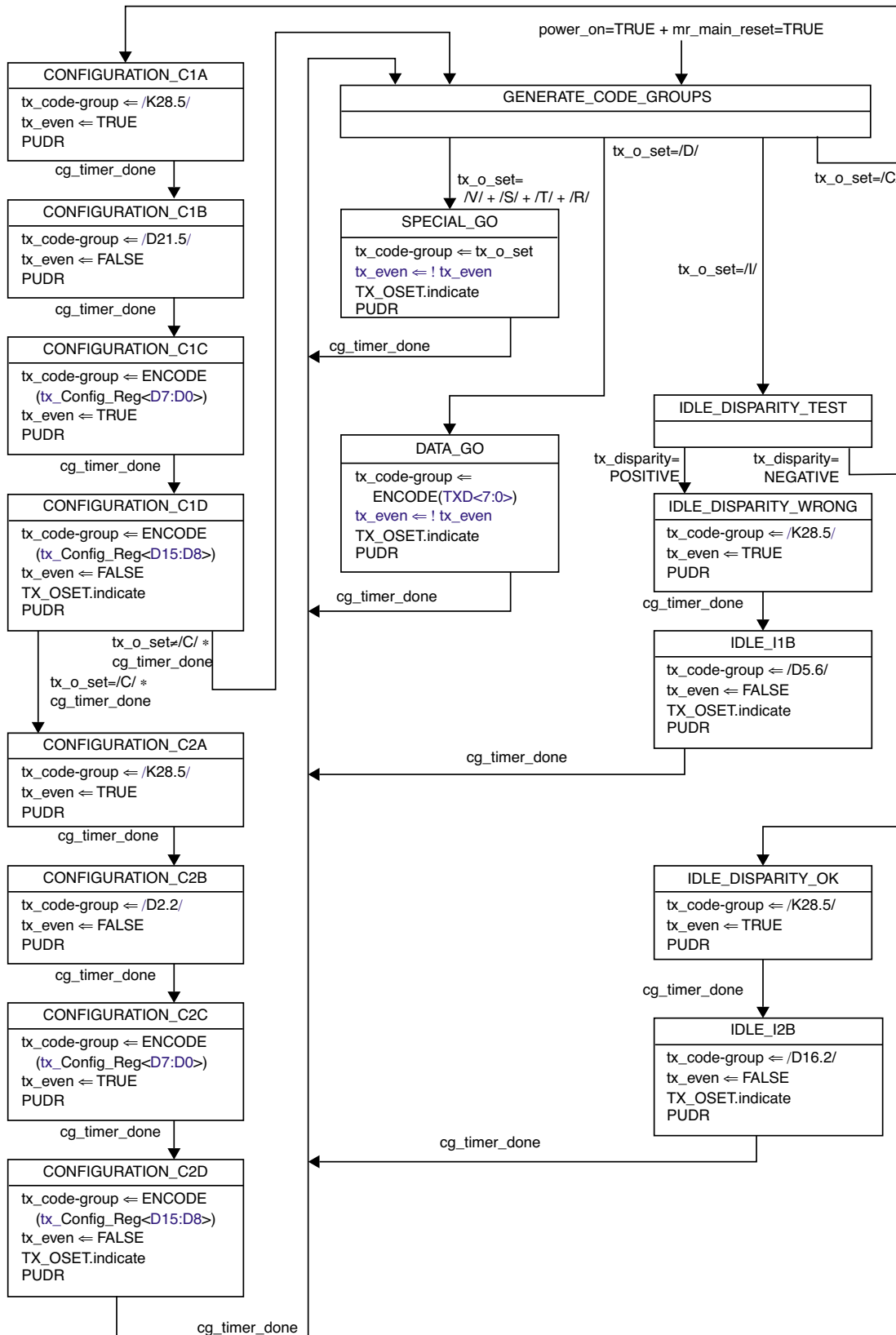
Figure 36–6—PCS transmit code-group state diagram
