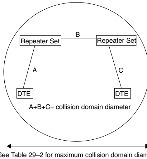
Figure 29-5—System Model 1: Two Class II repeaters
