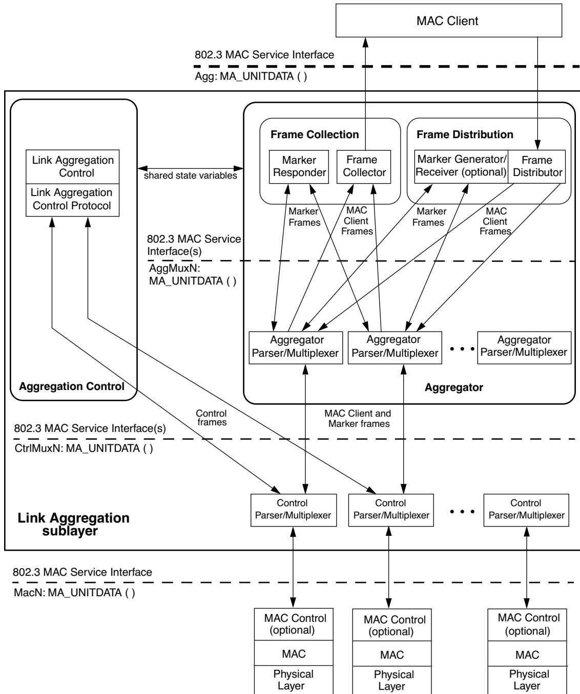
Figure 43-2—Link Aggregation sublayer block diagram
