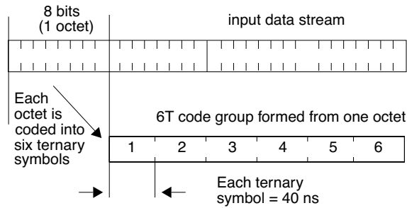
Figure 23–4—8B6T coding
